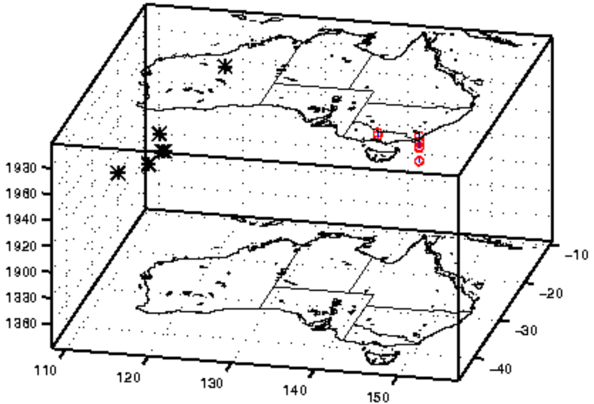
FIG. 9. Alarm Cube of the zones with anomalous decrease in seismic rate in Australia.
